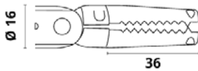
Alligator jaws GR 16
