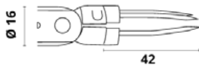
Three finger jaws GR 16
